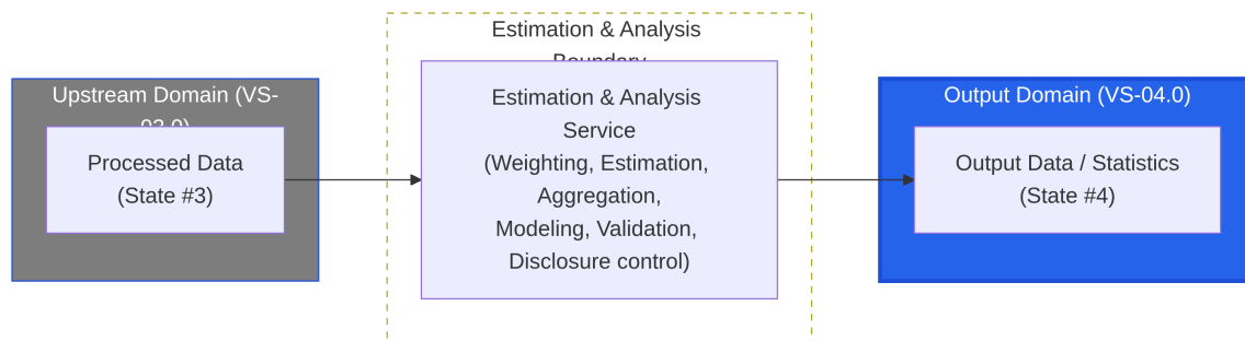
Figure 2: Steady State Transition from Processed Data to Output Data through the estimation and analysis service at the domain boundary. State #4 is shared with VS-05.0 Statistical Product Composition.
