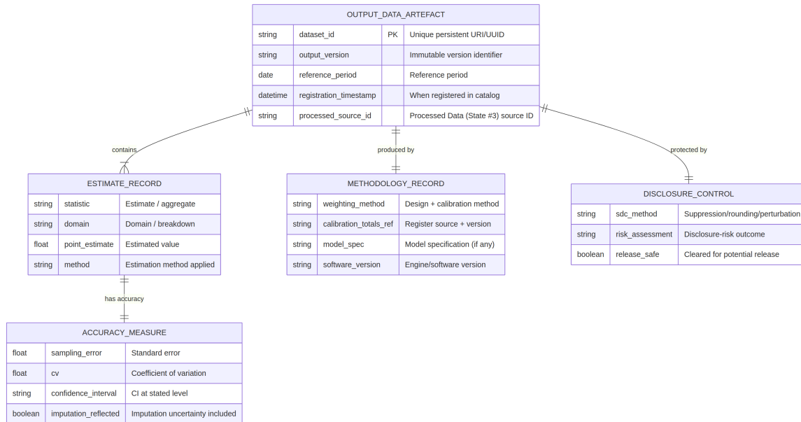
Figure 7: Output Data Artefact Structure. Reading guide: each box is a type of record with its fields; a connecting line means the records are linked. Each output version contains estimates with accuracy measures, is linked to the methodology that produced it and the applied disclosure control, and is traceable to the processed source data.
