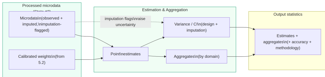
Figure 6: Estimation and Aggregation Architecture. Calibrated weights and imputation-flagged microdata feed point estimation and aggregation; variance estimation reflects both the survey design and the imputation uncertainty, and every output carries its accuracy and methodology.
