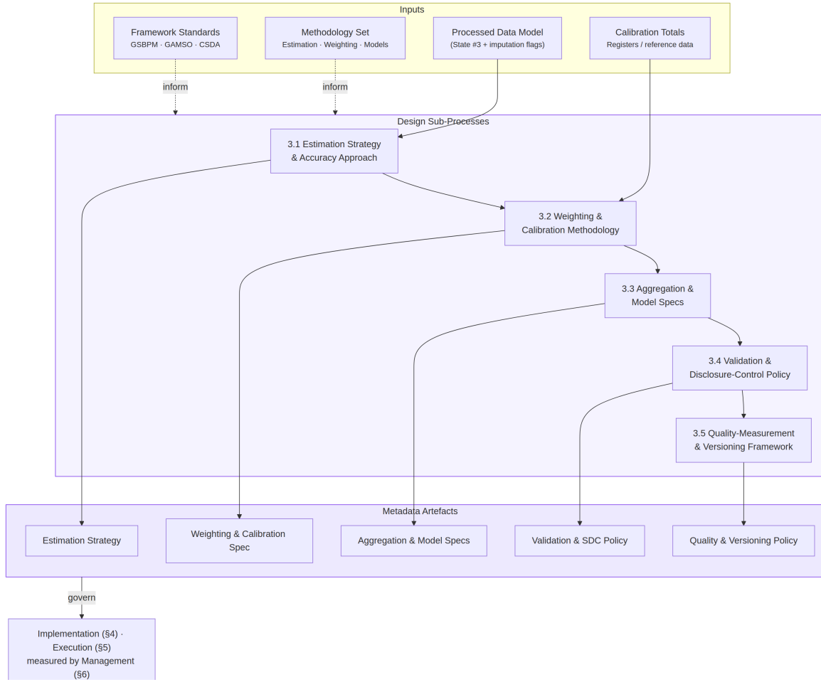
Figure 4: Design Process Decomposition. The processed data model, methodology set, calibration totals, and framework standards flow into five design sub-processes, producing metadata artefacts that govern Implementation, Execution, and Management.
