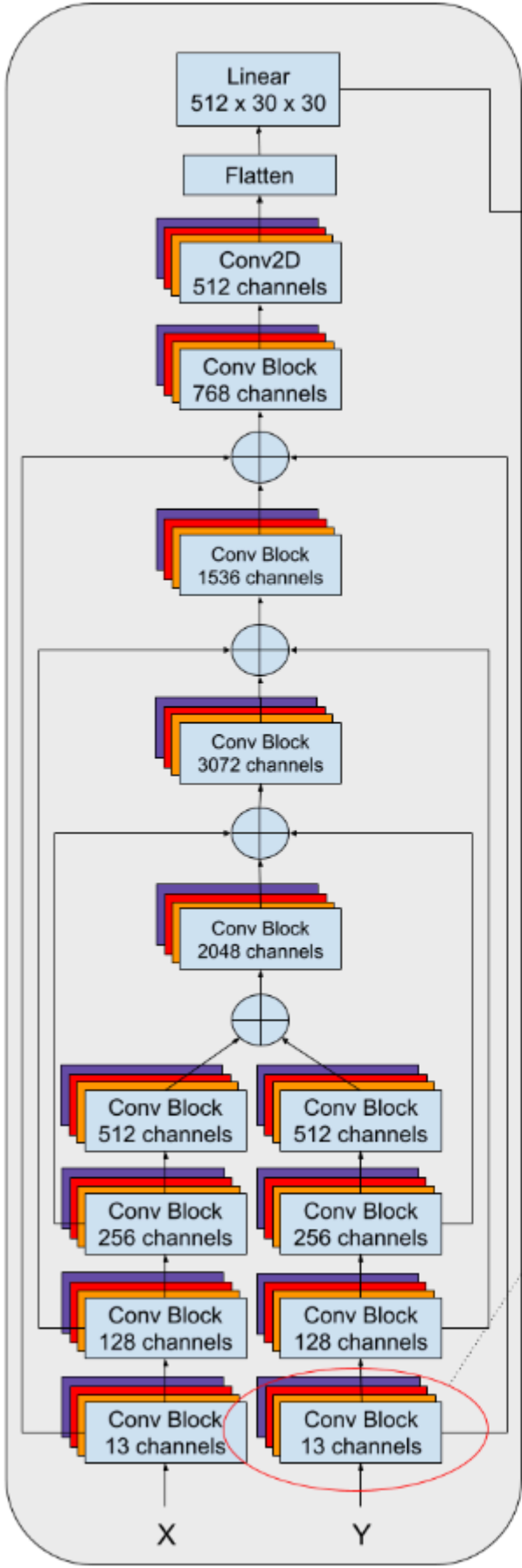
Convolutional Encoder Block
