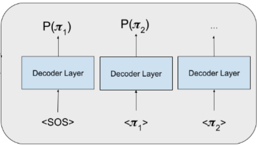
Transformer Decoder Block
