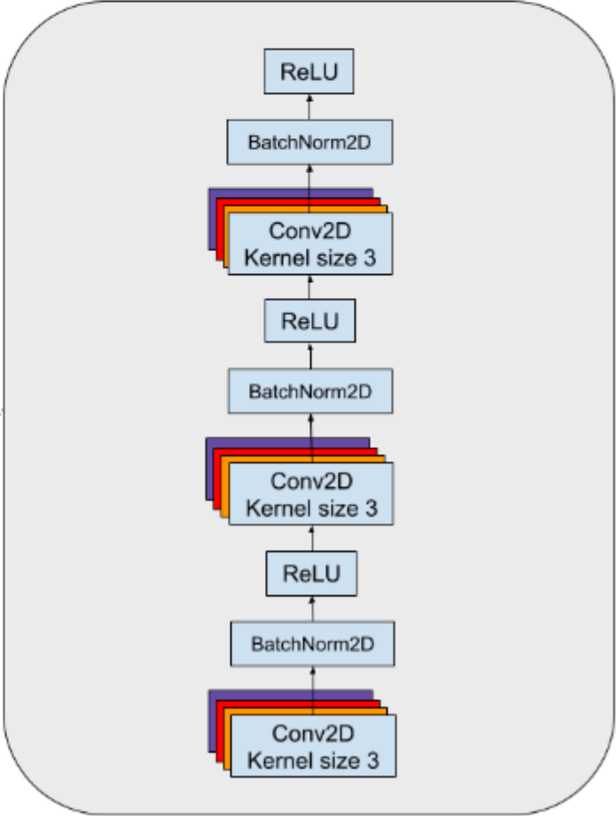
Conv Block
