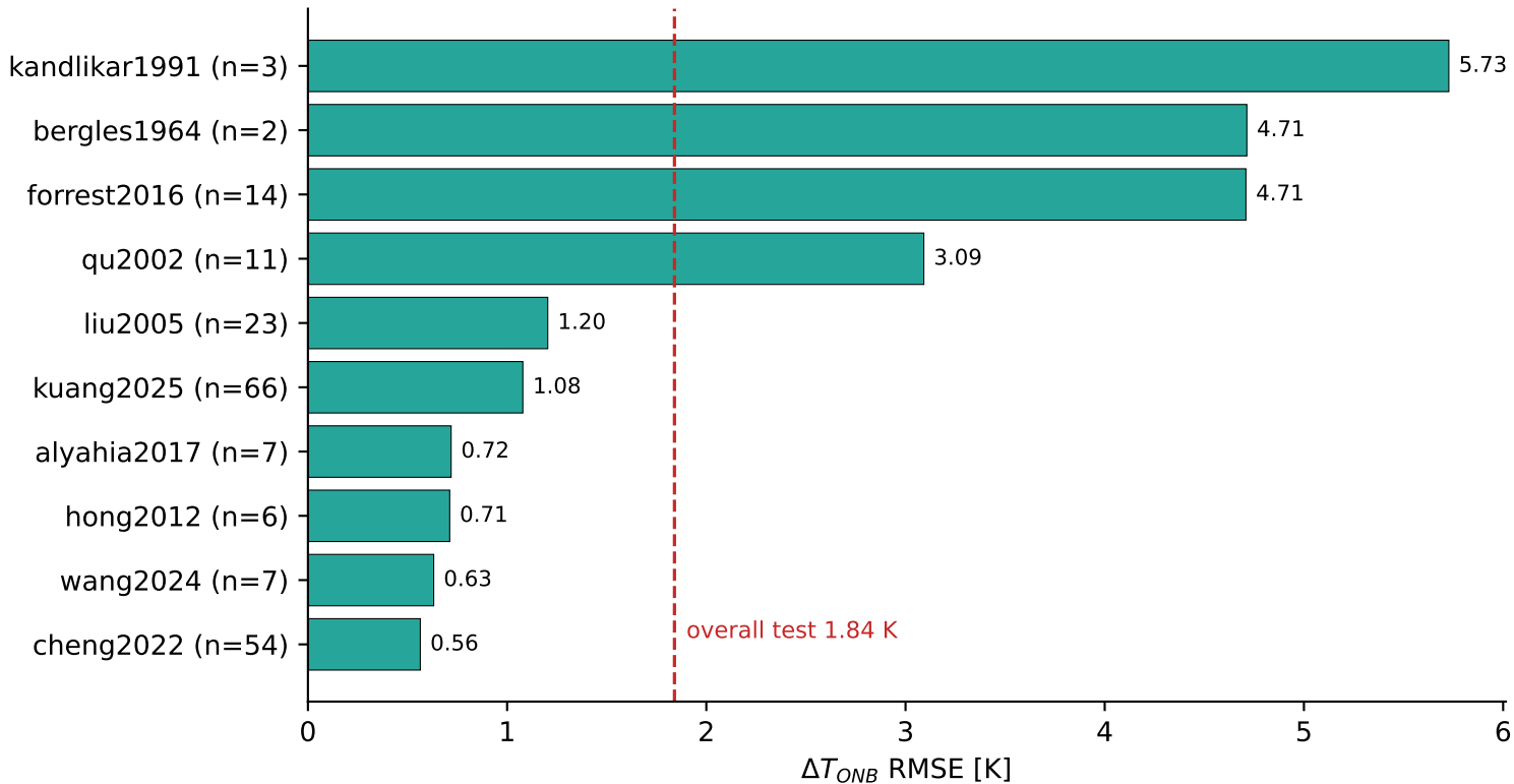
Per-source wall-superheat error (PINN v11, all data)
