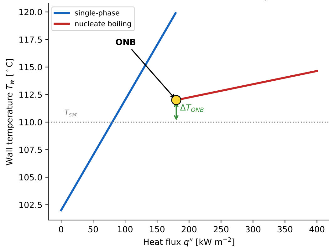
(a) ONB identification from the boiling curve
