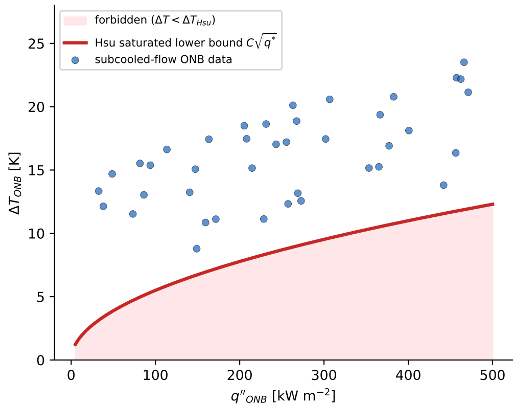
(b) Hsu criterion as a one-sided lower bound
