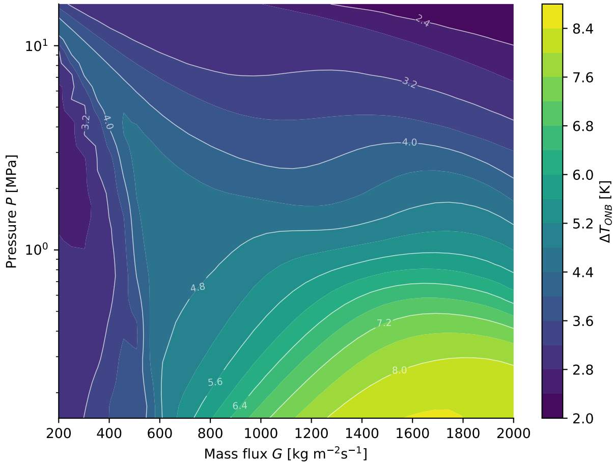
Design map: predicted \Delta T_{ONB} [K] (stainless, D_h=3 mm, \Delta T_{sub}=20 K, water)
