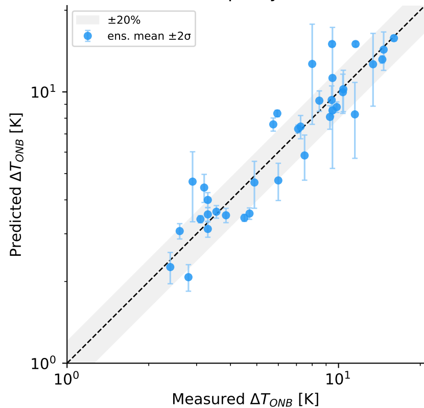
(a) Ensemble parity ( K=5, \pm 2\sigma )
