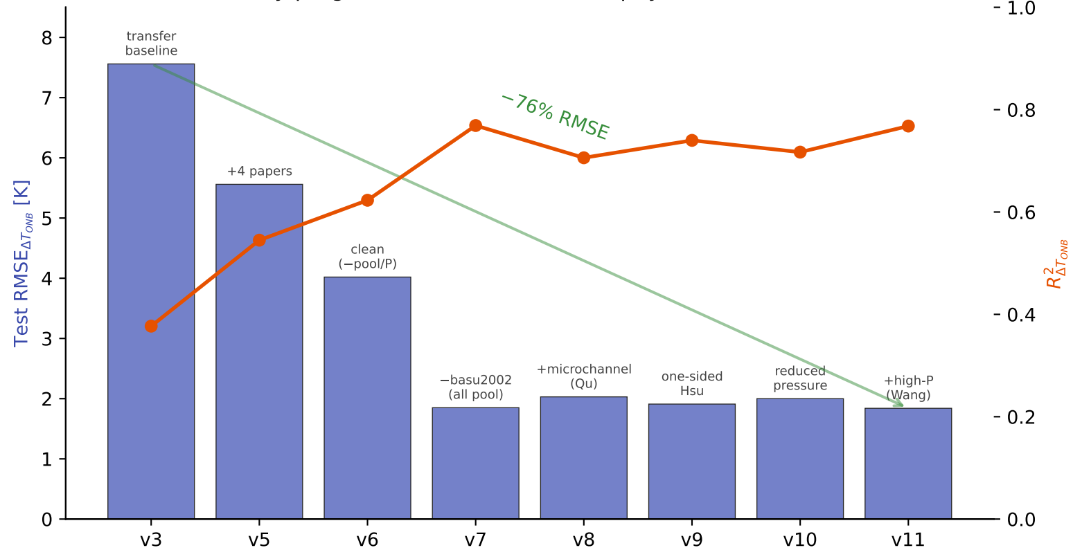
Accuracy progression: data curation + physics fixes (v3→v11)
