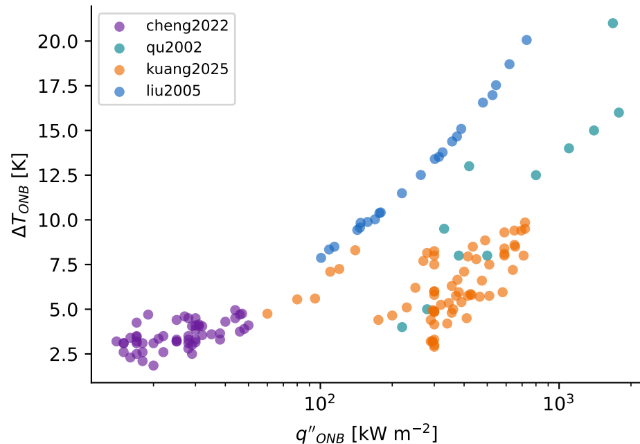
(b) Heat flux: q \uparrow \Rightarrow \Delta T_{ONB} \uparrow (data, r=0.6-0.9 )
