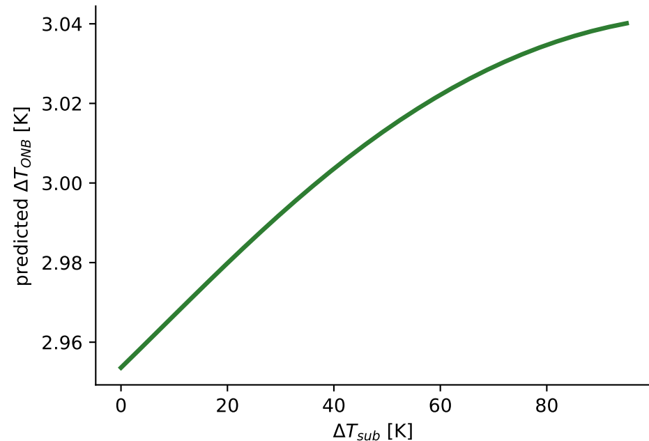
(a) Subcooling: \Delta T_{sub} \uparrow \Rightarrow \Delta T_{ONB} \uparrow (model)
