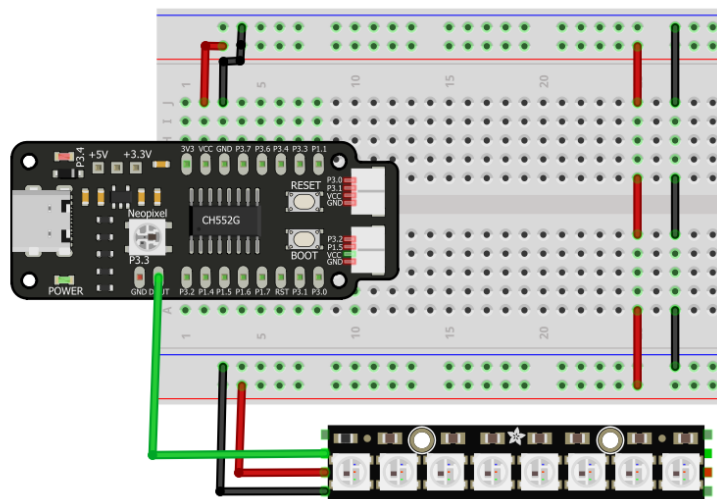
Figura 2.19: Tira LED WS2812
