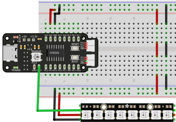
Figura 2.20: Tira LED WS2812
