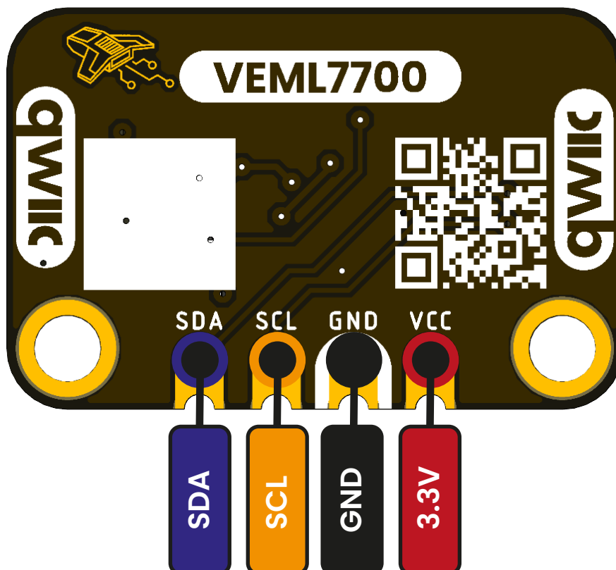
Bottom view
