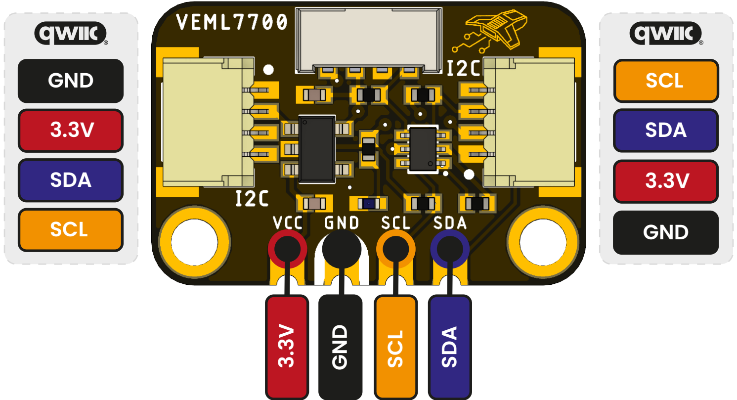
Top view
