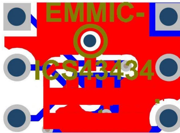
EMMIC-ICS43434 PCB – Bottom
