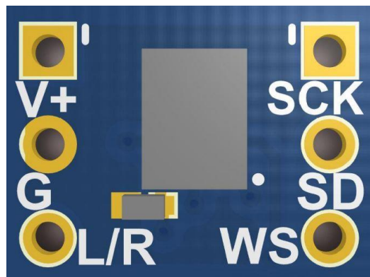
EMMIC-ICS43434 PCB – Top
