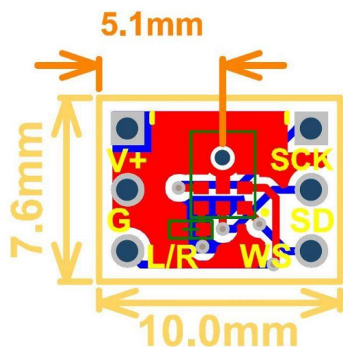
EMMIC-ICS43434 PCB – Top
