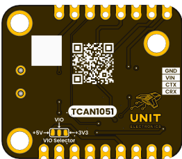
Underside components and connections
