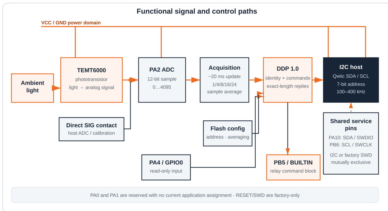
Figure 3.1 — Functional signal and control paths. The direct SIG branch and controller PA2 ADC observe the sensor path. DDP publishes the averaged sample through I2C and controls the internal PB5/BUILTIN indicator.
