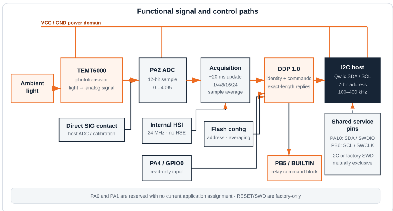
Figure 3.1 — Functional signal and control paths. The direct SIG branch and controller PA2 ADC observe the sensor path. Firmware averages the sample and publishes it through DDP over I2C. The internal HSI supplies the 24 MHz application clock; no HSE crystal or external clock is used.
