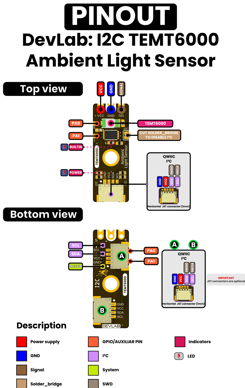
Figure 4.1 — Released general pinout for hardware revision V0.3.1.
