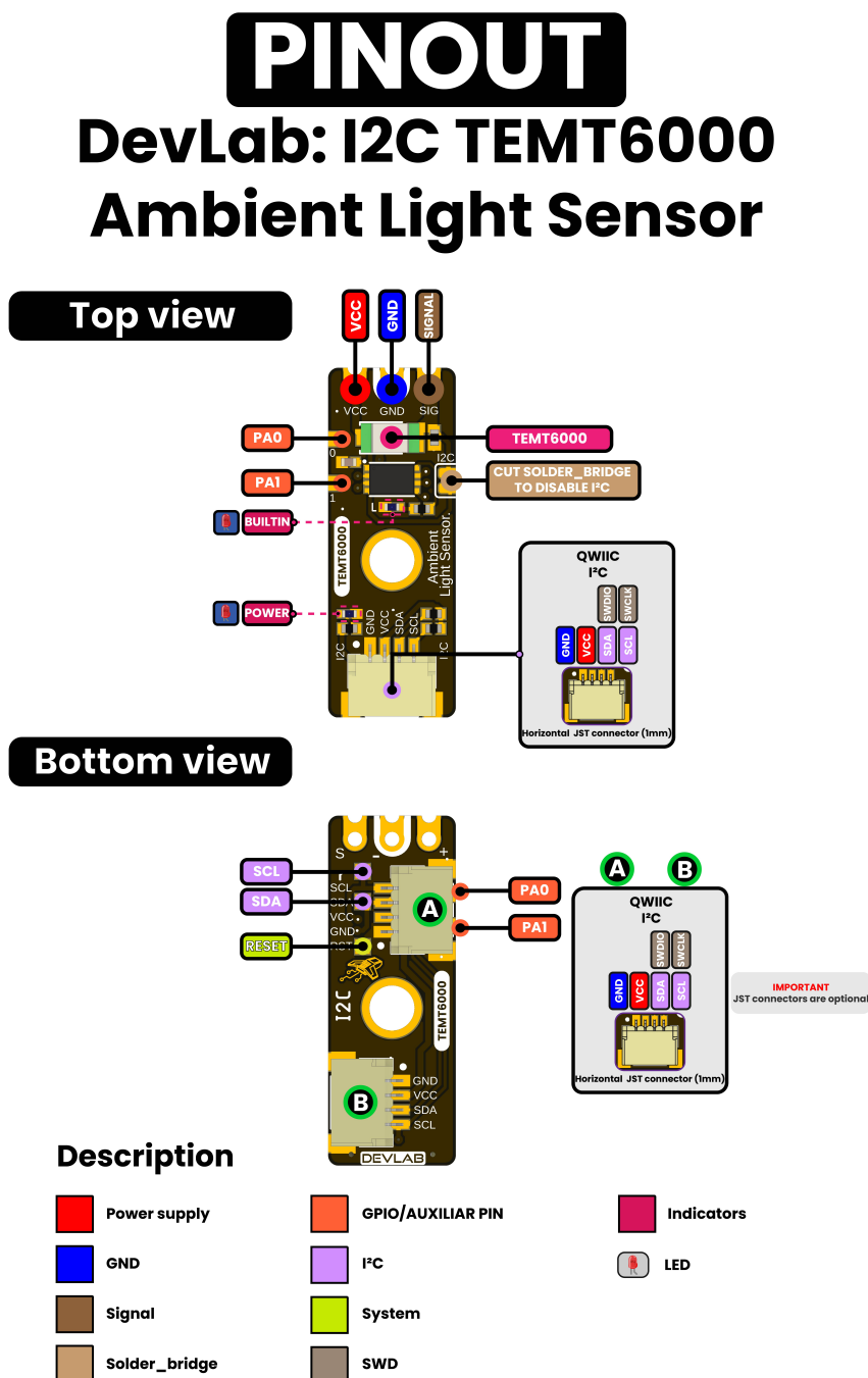
Figure 4.1 — Released general pinout for hardware revision V0.3.1.
