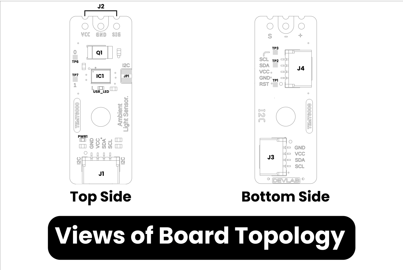
Figure 1.1 — V3.1.0 board topology with top- and bottom-side reference designators.
