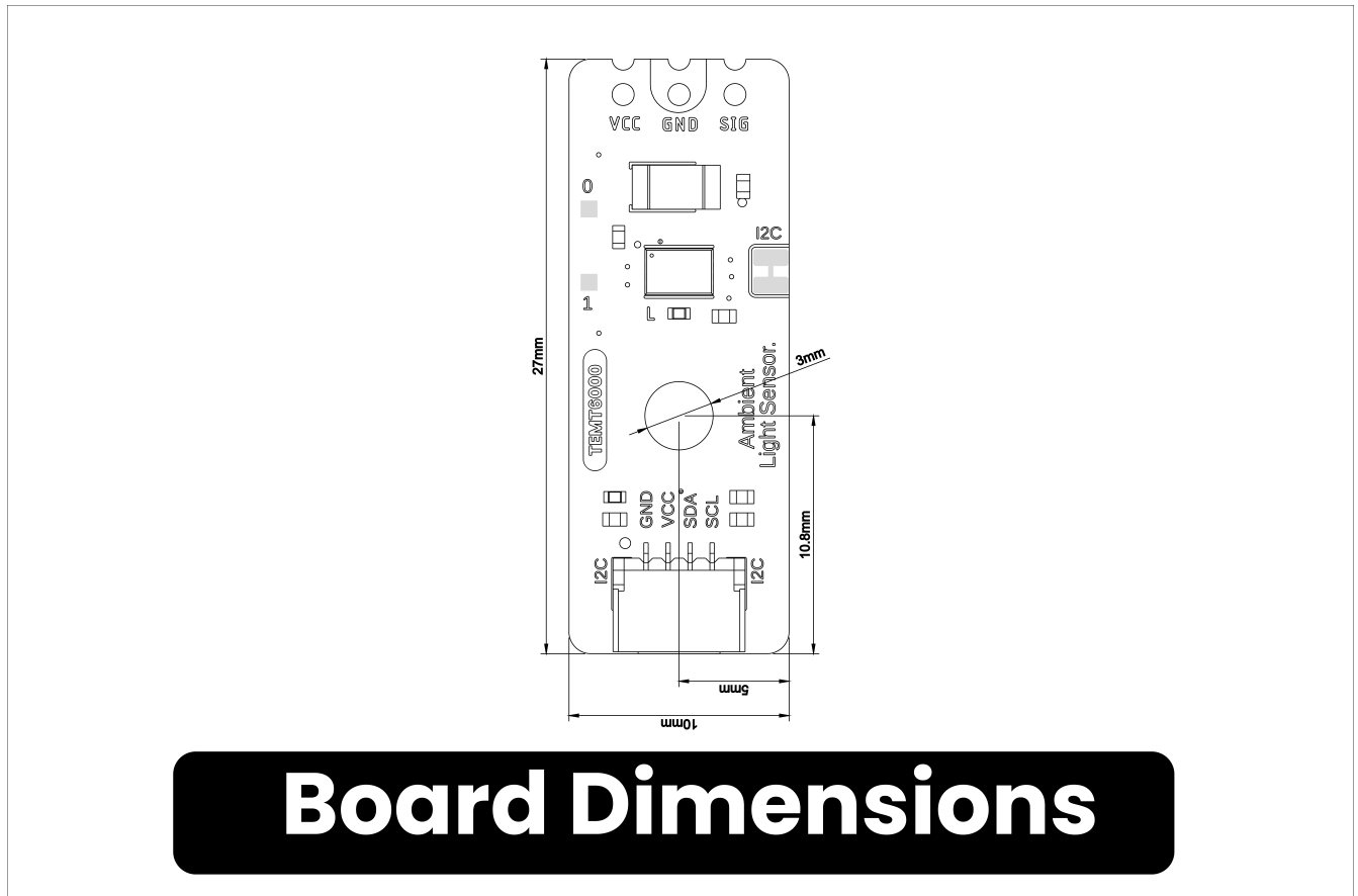
Figure 6.1 — V3.1.0 board dimensions.
