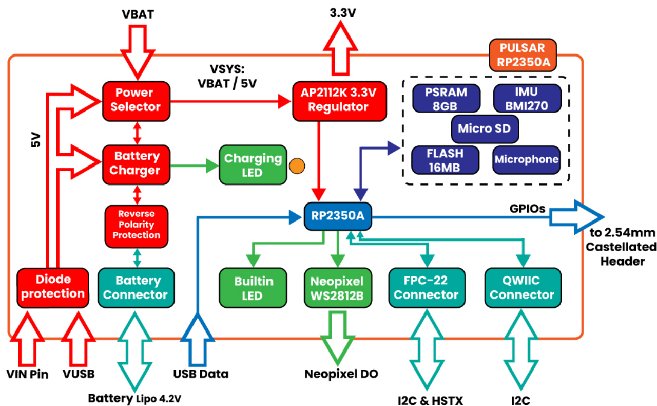
PULSAR RP2350A Block Diagram
