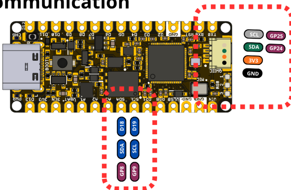
I2C and QWIIIC connections
