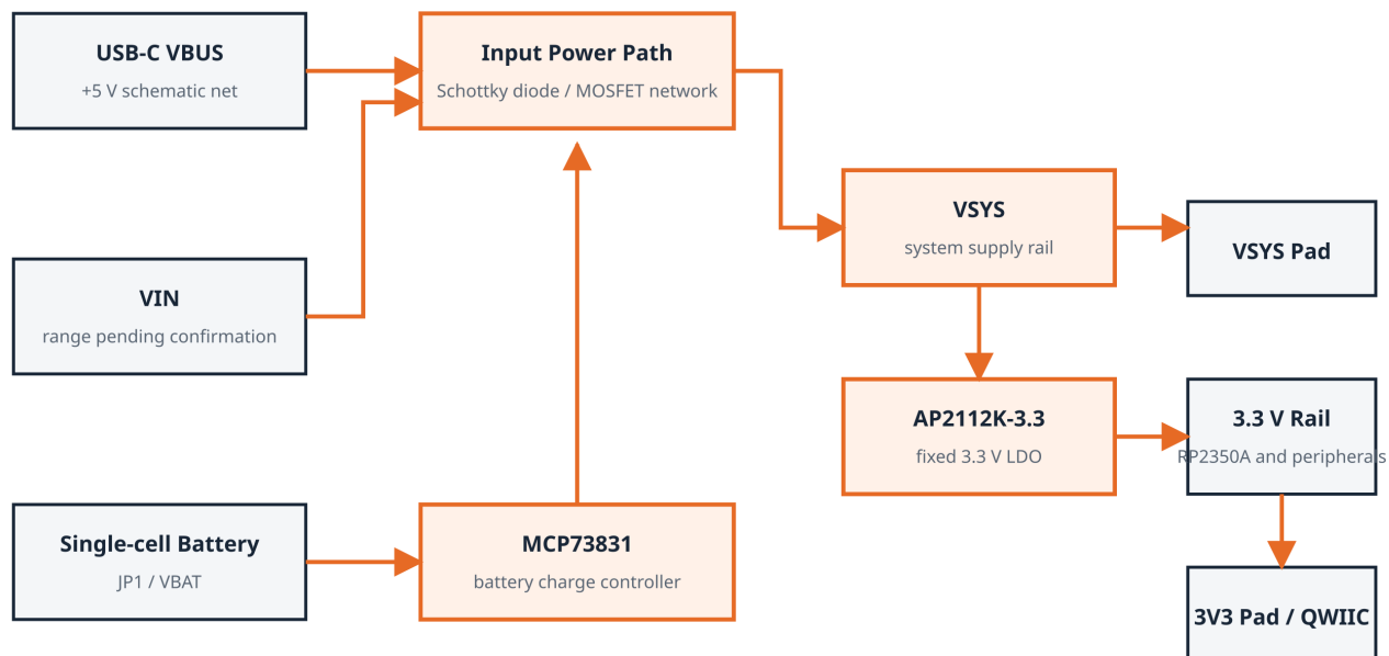
PULSAR RP2350A — Power Tree
