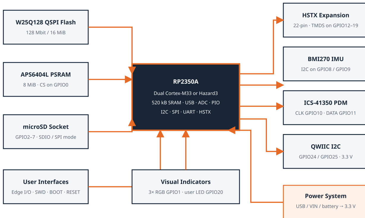
PULSAR RP2350A — Functional Block Diagram
