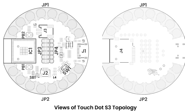
Fig. 3.3: Topology
