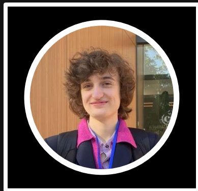
Julia
