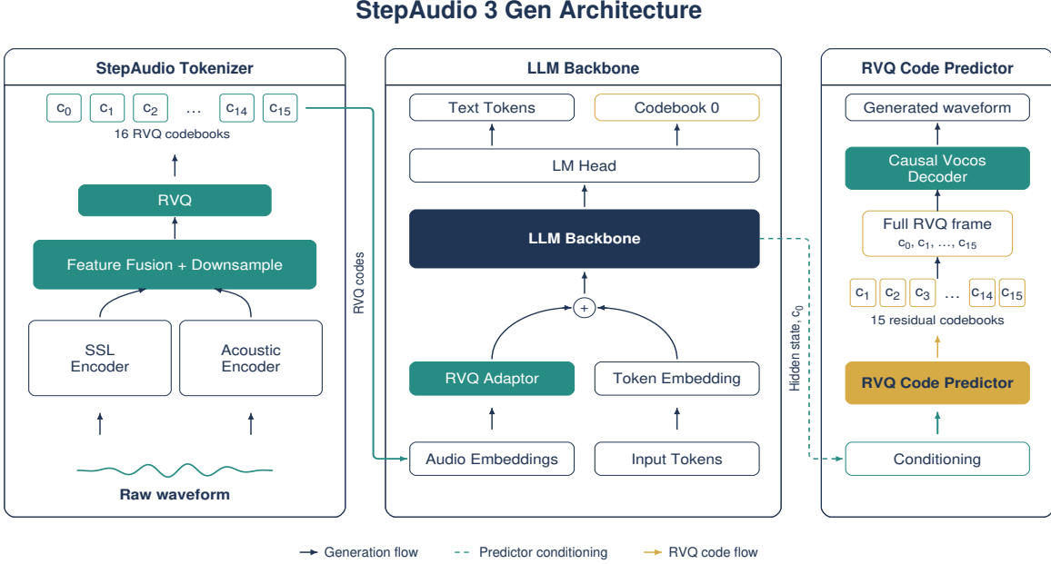
Figure 1: Overview of the StepAudio 3 Gen architecture. At each audio frame, the LLM predicts c_0 , and the RVQ Code Predictor conditions on the LLM hidden state and c_0 to predict c_1, \dots, c_{15} . All sixteen codes form the full RVQ frame used for waveform decoding. \oplus denotes element-wise addition: at audio positions, the RVQ Adaptor output is added to the corresponding token embedding (§2.2).
