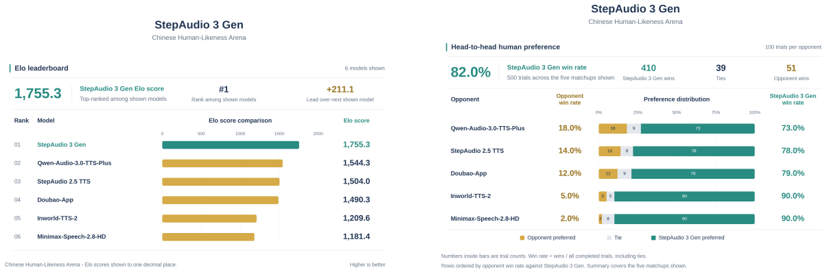
(a) Elo rankings of models on the Chinese human-likeness test set under human evaluation.
