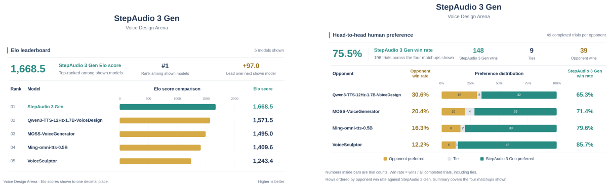
(a) Elo rankings of models on the voice design task under blind human evaluation. (b) Head-to-head results for StepAudio 3 Gen against baseline models on the voice design task.
