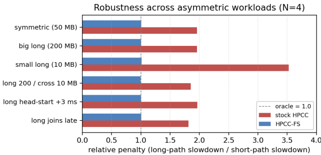
Fig. 4. Robustness across asymmetric-size and staggered-start variants at N = 4 . HPCC-FS is within 1.0 \pm 0.012 across all six scenarios, including the small-long worst case where stock reaches 3.53\times .
