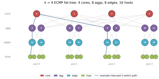
(b) k = 4 ECMP fat-tree (4 pods).
