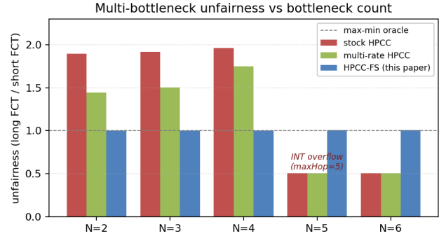
Figure 2: Multi-bottleneck unfairness vs bottleneck count N . HPCC-FS is flat \approx 1.0 across the entire sweep; stock and multi-rate HPCC fail at N \leq 4 and break at N \geq 5 (INT-overflow regime).
