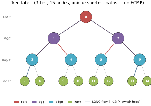
(a) Tree fabric — unique shortest paths, no ECMP.
