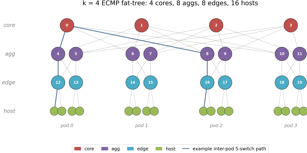
Figure 4: Canonical k = 4 ECMP fat-tree (4 cores, 8 aggs, 8 edges, 16 hosts in 4 pods). The highlighted line is a representative inter-pod 5-switch path.
