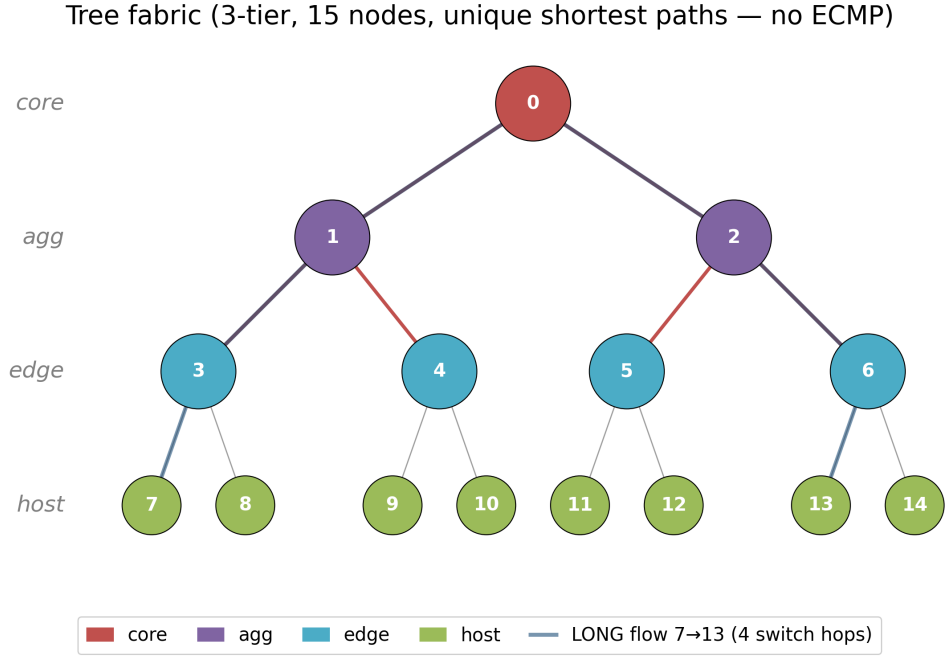
Figure 3: Tree-fabric topology (3-tier, 15 nodes, unique shortest paths — no ECMP). The highlighted line is the long flow 7 \rightarrow 13 , which crosses four switches.
