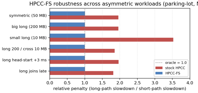
Figure 5: Robustness across asymmetric-size and staggered-start variants at N = 4 . HPCC-FS is within 1.0 \pm 0.012 across all six scenarios, including the small-long worst case where stock reaches 3.53\times .
