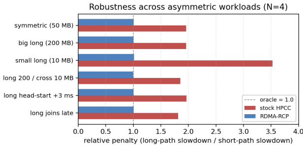
Figure 4: Asymmetric-size and staggered-start variants at N=4 : RDMA-RCP within 1.0 \pm 0.012 in all six; stock reaches 3.53\times (small-long).
