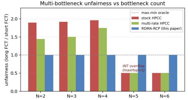
Figure 2: Multi-bottleneck unfairness vs bottleneck count N . RDMA-RCP is flat \approx 1.0 across the entire sweep; stock and multi-rate HPCC fail at N \leq 4 and break at N \geq 5 (INT-overflow regime).
