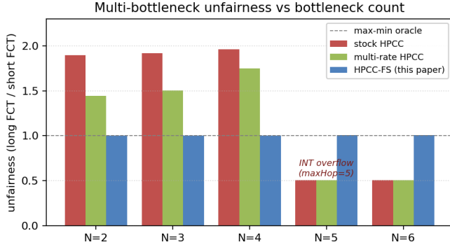
Fig. 2. Multi-bottleneck unfairness vs bottleneck count N . HPCC-FS is flat \approx 1.0 across the entire sweep; stock and multi-rate HPCC fail at N \leq 4 and break at N \geq 5 (INT-overflow regime).
