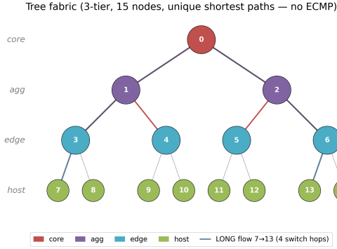
(a) Tree fabric — unique shortest paths, no ECMP.
