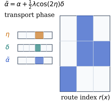
Figure 1: Fixed geometric routing mechanism. A normalized representation is projected onto a fixed 4D chart, written as paired complex coordinates, decomposed into Hopf base coordinates and a fiber phase, transport-corrected along the phase coordinate, and discretized into sector bins. Concentrated routing occurs when the resulting bins receive uneven occupancy across the representation distribution.
