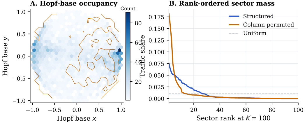
Figure 3: Proxy-side occupancy and sector concentration support. Structured states occupy the Hopf base unevenly, and sector mass is more concentrated than under the column-permuted control.
