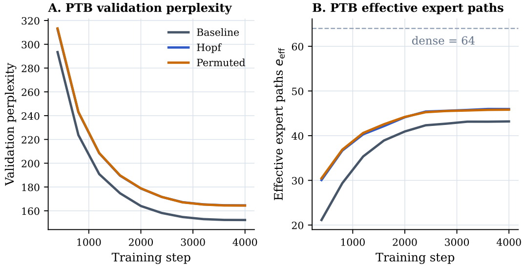
Figure 4: PTB training dynamics for validation perplexity and effective expert-path usage. Hopf and permuted fixed routing remain close throughout training.
