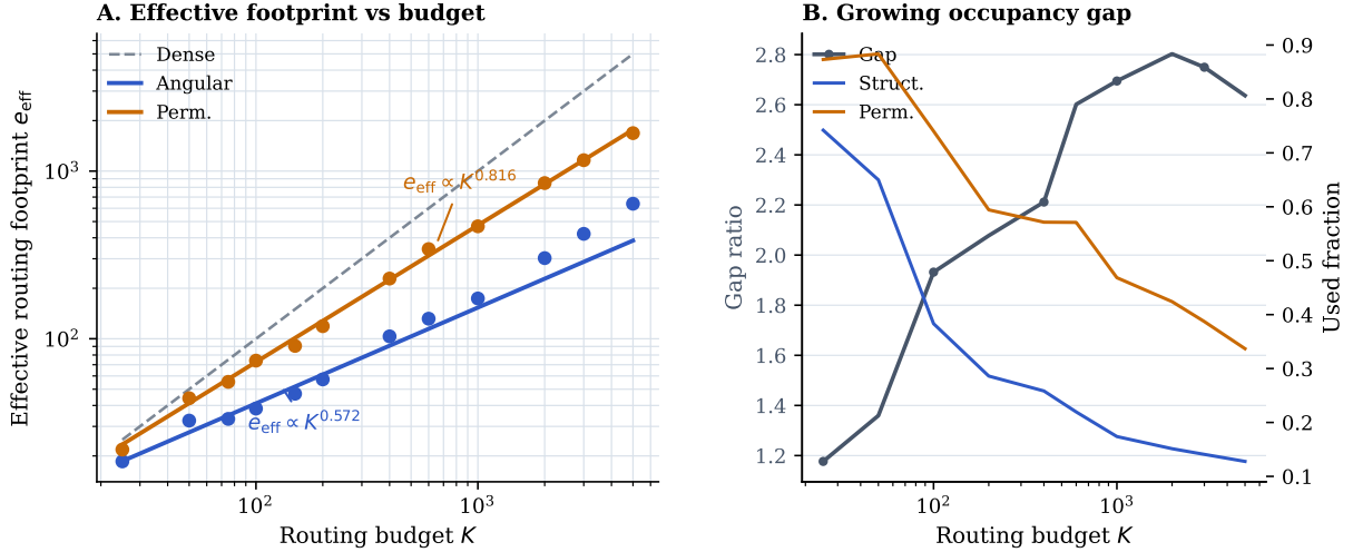
Figure 2: Main proxy scaling result. Left: the effective routing footprint of the fixed angular map grows sublinearly with routing budget, unlike dense routing and the permuted fixed-routing control. Right: the occupancy gap widens with K , indicating that the structured proxy uses a shrinking fraction of available routing cells.
