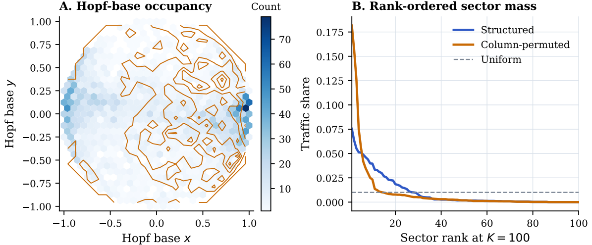
Figure 2: Why a fixed angular partition can behave like a sparse router. Left: the structured proxy occupies the Hopf base unevenly, whereas the column-permuted control is more diffuse. Right: after sectorization at K = 100 , the structured proxy places much more traffic in the top-ranked sectors. This is the geometric intuition behind the sublinear routing footprint measured in the next figure.
