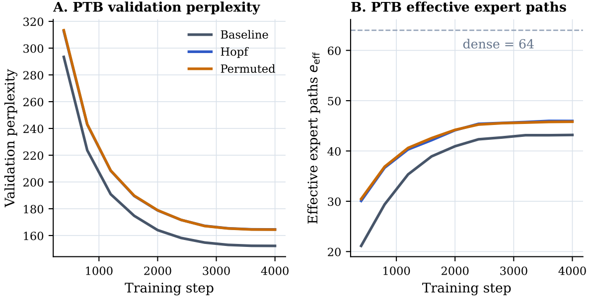
Figure 4: PTB training dynamics. The fixed Hopf and permuted route maps remain close throughout training on both validation perplexity and effective expert-path usage. This is the trainable version of the paper’s central negative result: the fixed routing effect transfers, but the specific geometry does not retain a quality advantage once experts co-adapt.
