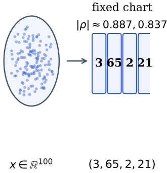
Figure 1: Fixed geometric routing mechanism. A normalized representation is projected onto a fixed 4D chart, written as paired complex coordinates, decomposed into Hopf base coordinates and a fiber phase, transport-corrected along the phase coordinate, and discretized into sector bins. Concentrated routing occurs when the resulting bins receive uneven occupancy across the representation distribution.
