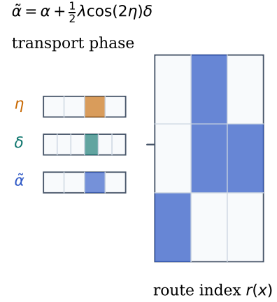
Figure 1: Fixed geometric routing mechanism. A normalized representation is projected onto a fixed 4D chart, written as paired complex coordinates, decomposed into Hopf base coordinates and a fiber phase, transport-corrected along the phase coordinate, and discretized into sector bins. Concentrated routing occurs when the resulting bins receive uneven occupancy across the representation distribution.
