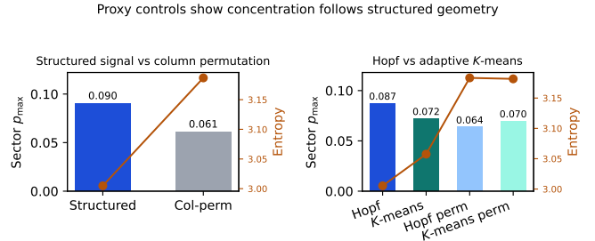
Figure 3: Proxy-side control figure. Left: concentration weakens when structured embeddings are column-permuted before routing. Right: fixed Hopf routing is more concentrated than adaptive K -means on the same proxy, and both families weaken under permutation controls. Bars show sector p_{\max} ; orange lines show sector entropy.
