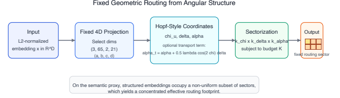
Figure 1: Fixed routing mechanism used in Paper 1. A normalized representation is projected onto a fixed 4D subspace, expressed in Hopf-style angular coordinates, optionally transport-corrected, and discretized into a sector under routing budget K . The positive proxy result is that structured embeddings occupy these sectors non-uniformly.
