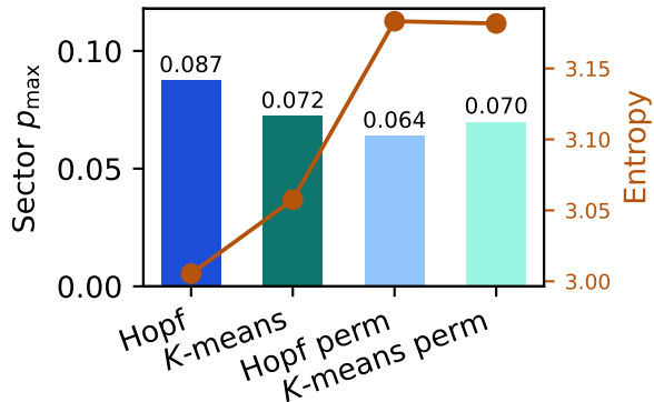
Hopf vs adaptive K-means
