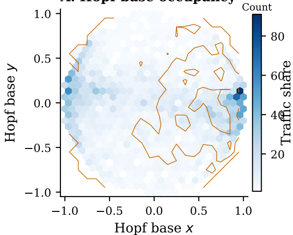
A. Hopf-base occupancy
