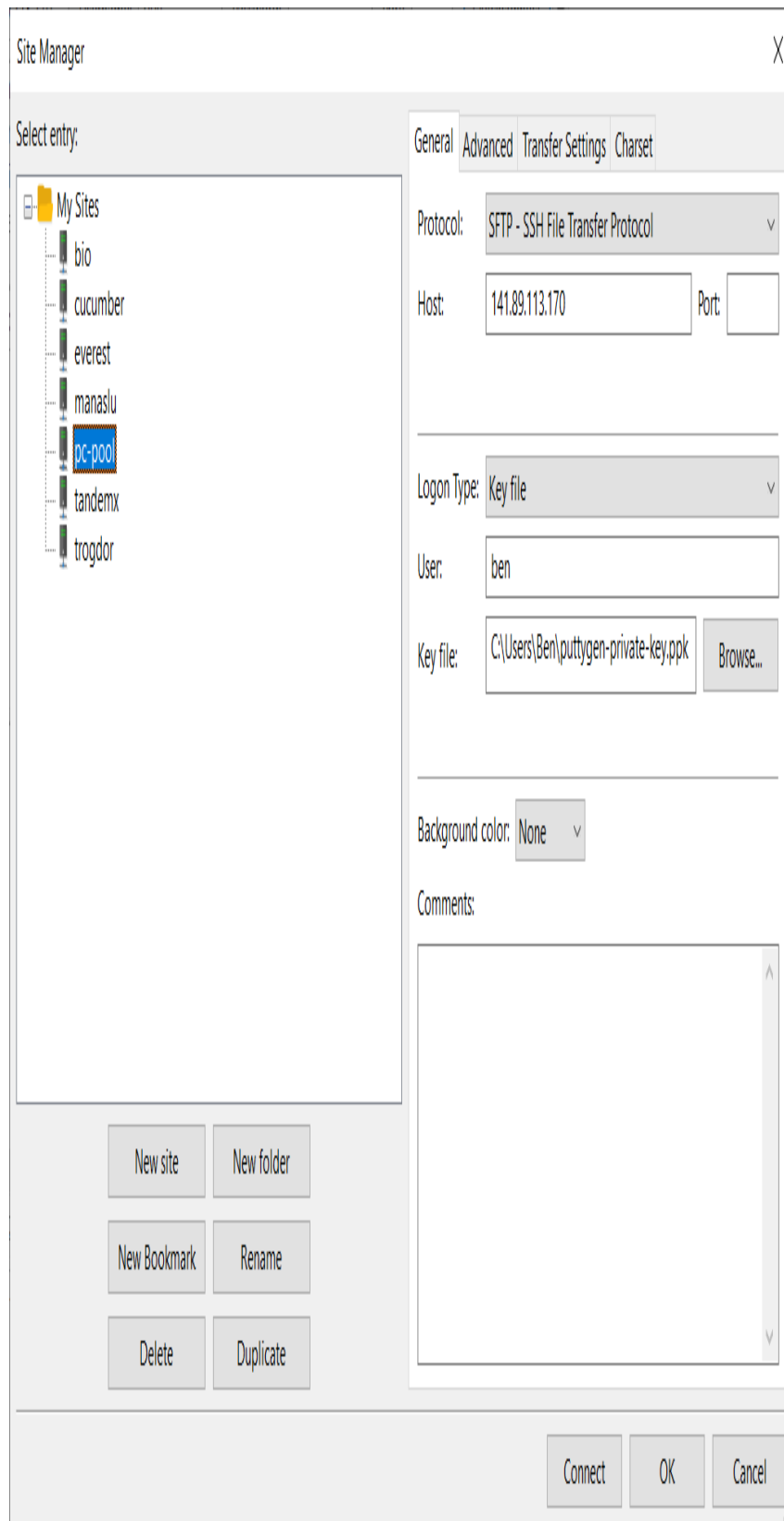
Figure 1: Open a FileZilla session and create a new site to the remote pc-pool host with your username and SSH private key.
