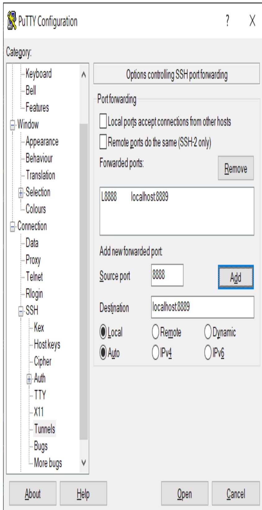
Figure 3: Port forwarding in PuTTY.
