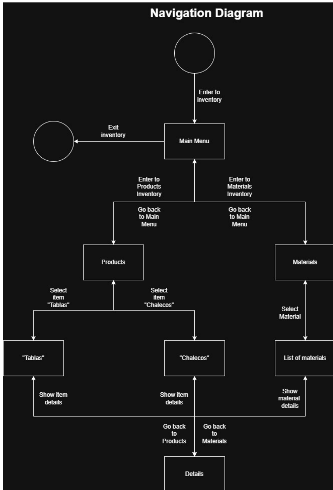
Figure 8: Navigation Flow Diagram for KAVEM System
