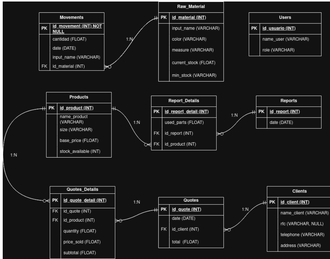
Figure 2: Entity-Relationship Diagram for Sprint #1
