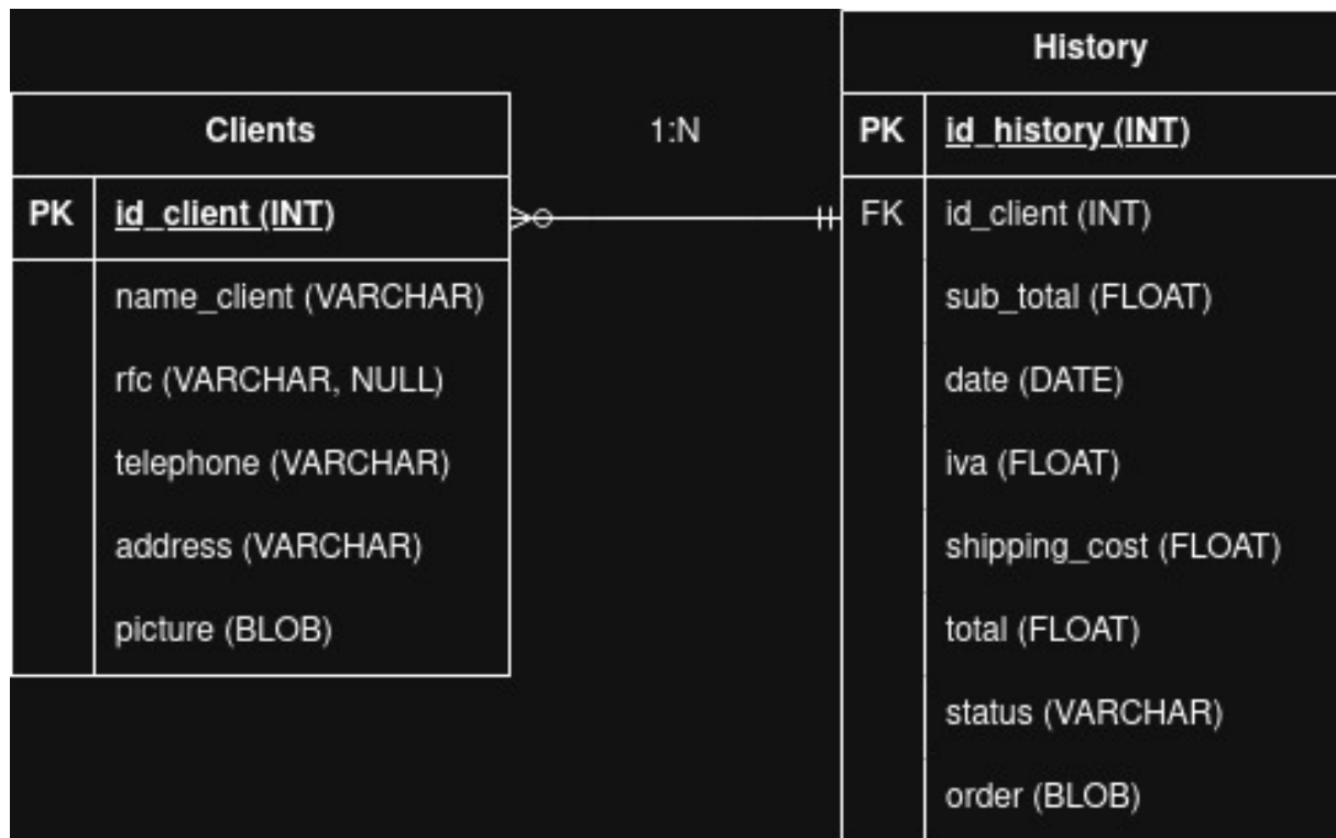
Figure 3: Entity-Relationship Diagram for Client Management Module
