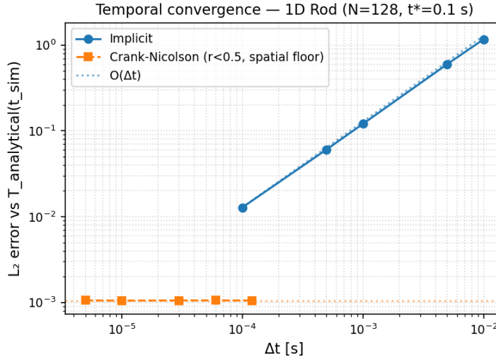
Figure 6: Temporal convergence study (1D rod, N = 128 , CG solver, q_V = 200 \text{ W m}^{-3} ). L_2 error vs. transient analytical solution at t^* = 0.1 \text{ s} as a function of \Delta t on a log-log scale. Implicit: first-order convergence ( \sim O(\Delta t) ). Crank-Nicolson: flat curve at the spatial accuracy floor ( L_2 \approx 1.05 \times 10^{-3} ), indicating that the CN temporal error is negligible for all stable \Delta t values at this mesh.
