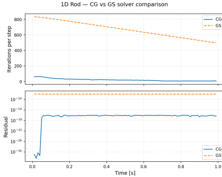
Figure 4: Performance comparison between Gauss-Seidel (GS) and Conjugate Gradient (CG) solvers on the 1D rod case ( N = 64 , \Delta t = 0.01 s, implicit, q_V = 200 \text{ W m}^{-3} ). Top: number of inner iterations per time step. Bottom: solver residual \|\mathbf{b} - \mathbf{A}\mathbf{T}\| at convergence. CG converges in \approx 32\times fewer iterations than GS due to the SPD structure of the diffusion matrix.
