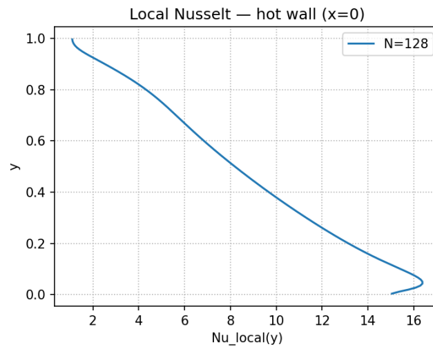
Figure 24: Local Nusselt number Nu(y) along the hot wall ( x = 0 ) at Ra = 10^6 and N = 128 . The sharp peak near y = 0 reflects the thin thermal boundary layer at the base of the hot wall where the cold fluid arrives from the bottom recirculation.
