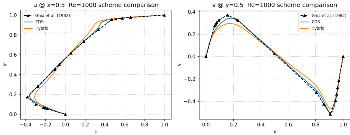
Figure 19: Comparison of computed centreline velocity profiles (CDS and Hybrid) against reference values of Ghia et al. [?] at Re = 1000 . Left: u -velocity along x = 0.5 . Right: v -velocity along y = 0.5 .
