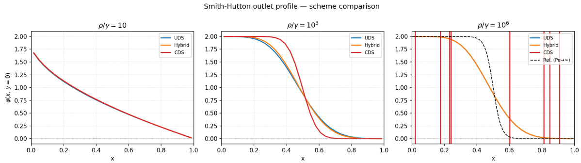
Figure 14: Exit profile \phi(x, 0) for CDS, UDS, and Hybrid compared against the reference of Smith and Hutton [?] at each \rho/\Gamma case. For \rho/\Gamma = 10^6 the reference corresponds to the Pe \rightarrow \infty limit.
