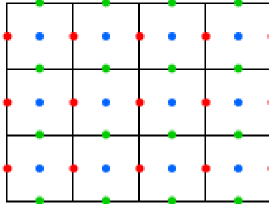
Figure 16: Staggered mesh layout. Pressure nodes (blue) are located at cell centres; u -velocity nodes (red) at east/west face midpoints; v -velocity nodes (green) at north/south face midpoints.
