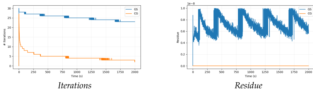
Figure 3: Performance comparison between Gauss-Seidel and Conjugate Gradient solvers. Number of iterations until solution (left) and solver residual after convergence (right).
