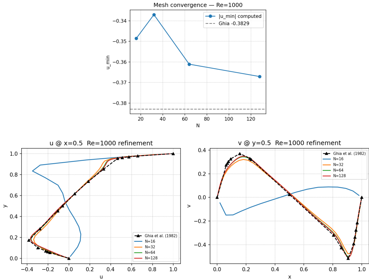
Figure 17: Mesh refinement study for the Lid-Driven Cavity ( Re = 1000 , CDS). Top: minimum u -velocity u_{\min} at x = 0.5 as a function of N , compared against the Ghia reference. Bottom: centreline u (left) and v (right) profiles at each mesh level.
