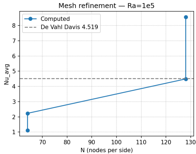
Figure 22: Mesh refinement study for the Differentially Heated Cavity ( Ra = 10^5 ). Average Nusselt number \overline{Nu} at the hot wall as a function of nodes per side N , compared against the de Vahl Davis reference [?].
