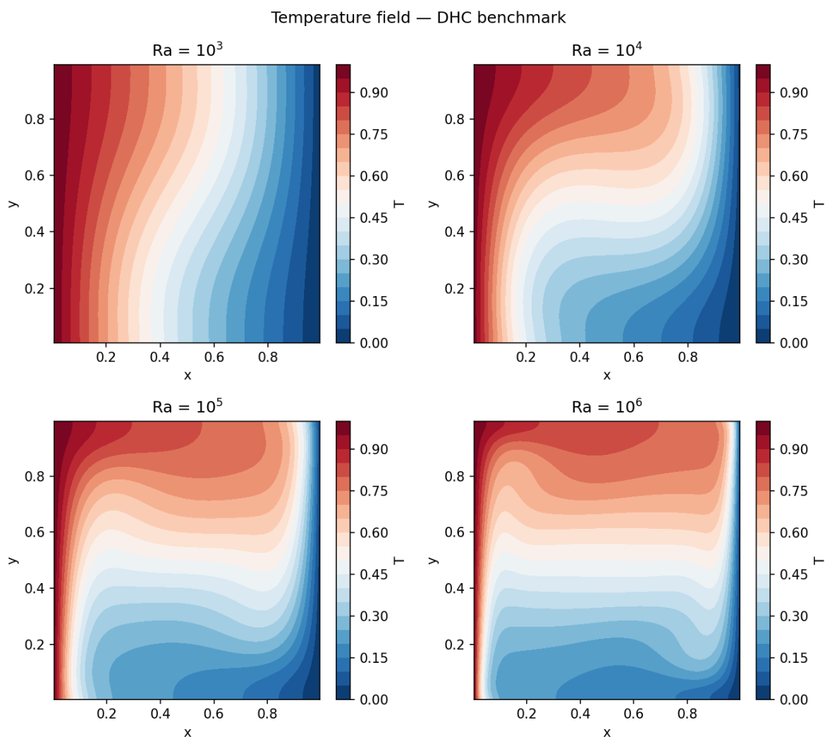
Figure 25: Steady-state temperature distribution for each Rayleigh number case. The growing asymmetry of the isotherms from Ra = 10^3 (near-linear conduction profile) to Ra = 10^6 (thin boundary layers on both walls) reflects the increasing dominance of convective transport.
