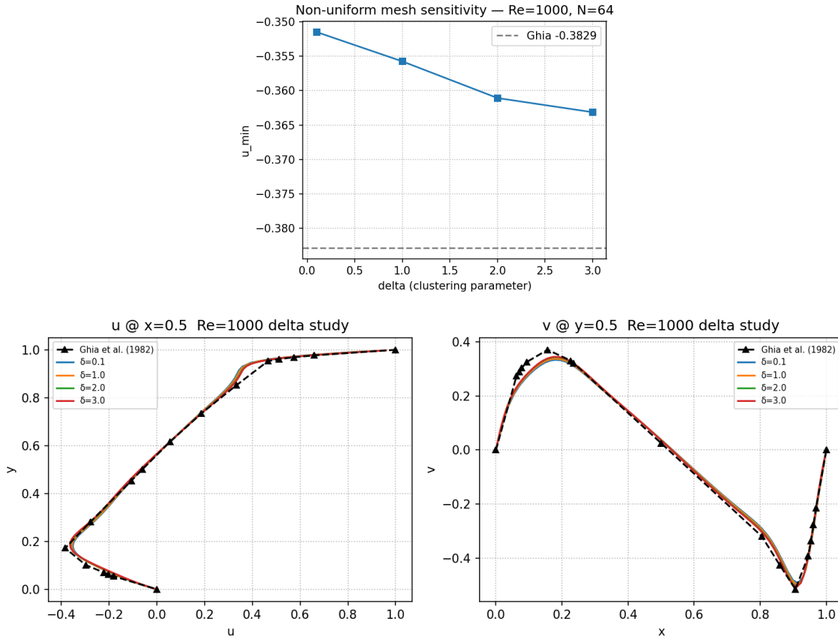
Figure 18: Non-uniform mesh sensitivity for the Lid-Driven Cavity ( Re = 1000 , N = 64 , CDS). Top: minimum u -velocity u_{\min} as a function of the clustering parameter \delta , compared against the Ghia reference. Bottom: centreline u (left) and v (right) profiles for each \delta value.
