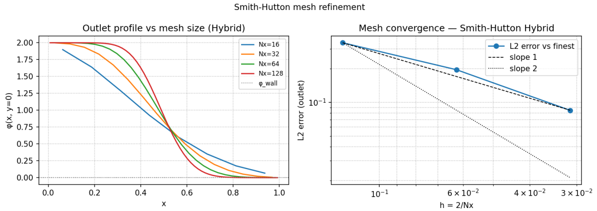
Figure 12: Mesh refinement study for the Smith-Hutton case ( \rho/\Gamma = 10^3 , Hybrid). Left: exit profile \phi(x, 0) for each mesh level. Right: L_2 error against mesh spacing h = 2/N_x ; reference slope lines indicate first- and second-order convergence rates.
