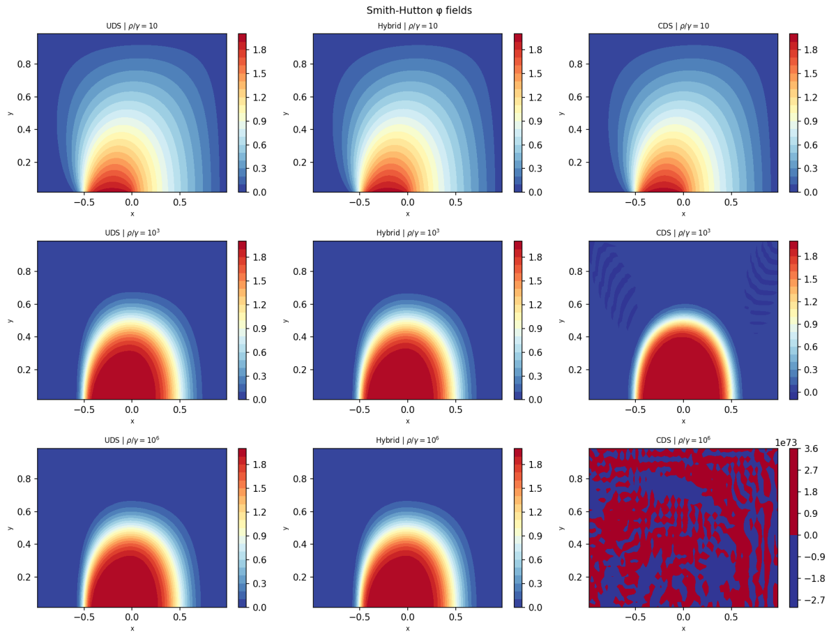
Figure 15: Steady-state \phi field for UDS (left column), Hybrid (centre column), and CDS (right column) across all three \rho/\Gamma cases (rows). At \rho/\Gamma = 10^6 the CDS solution has diverged and is shown at the scale of the numerical overflow.
