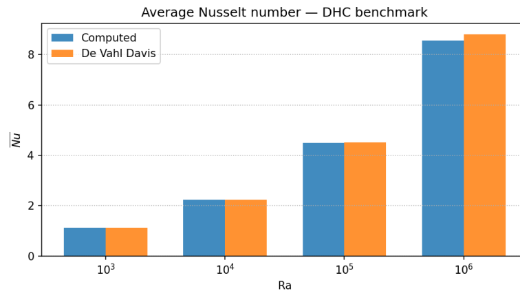
Figure 23: Average Nusselt number \overline{Nu} at the hot wall for each Rayleigh number case, compared against de Vahl Davis [?] benchmark values.
