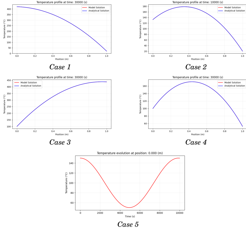
Figure 2.4: Comparison of model results with analytical solutions and implementation of mathematical expression reading for Dirichlet boundary condition.
