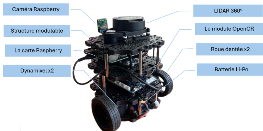
FIGURE 1 – Robot Turtlebot3 type burger
