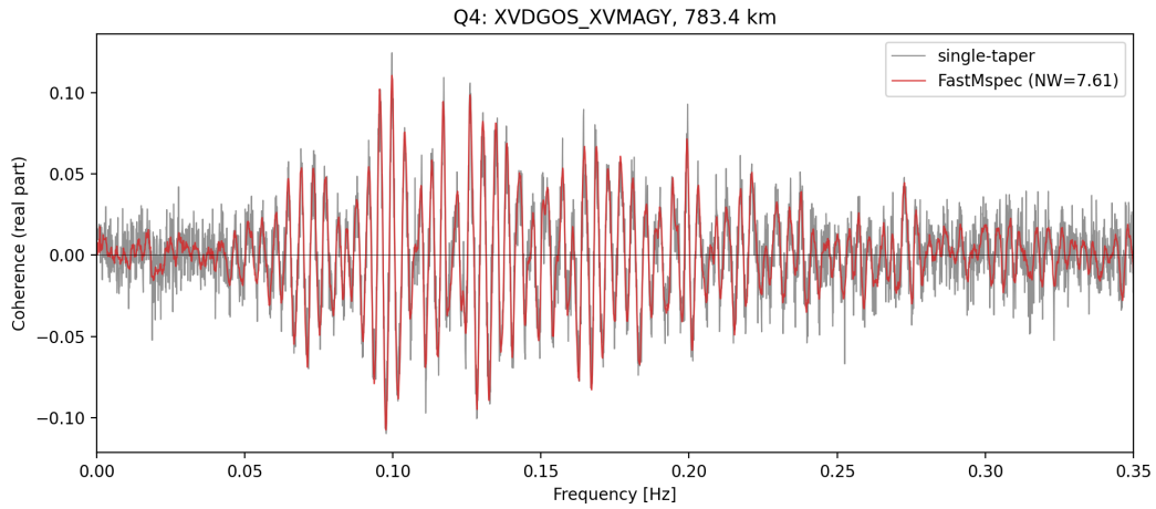
Figure 8: Quartile 4, FastMspec ( NW = 7.61 ) vs. single-taper, full band. A real, strong envelope is present, peaking around 0.09–0.13 Hz – corrects the impression from Figure 4's cropped view.
