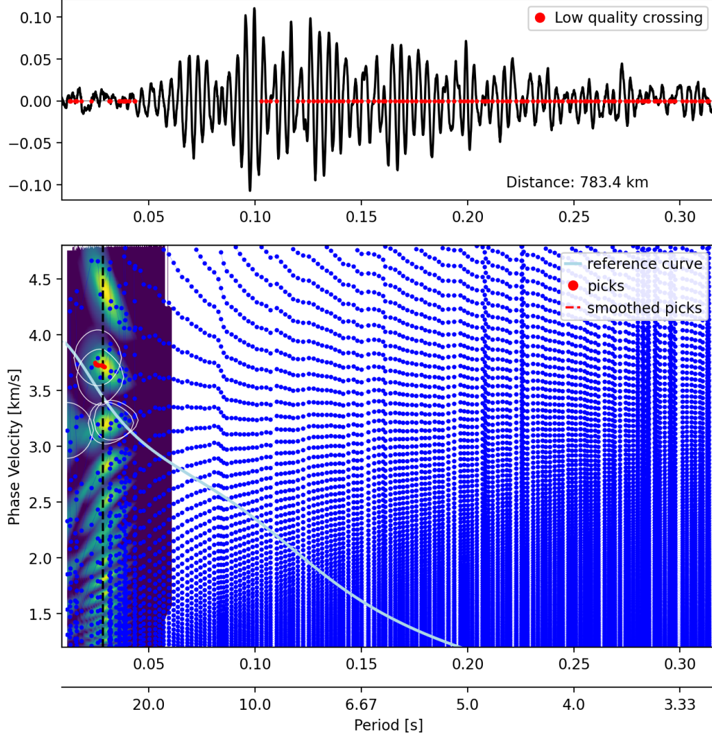
Figure 4: Quartile 4 (farthest), XVDGOS_XVMAGY, 783.4 km, NW = 7.61 ( 1.5 \times NW_{\text{high}} = 5.08 ; W \approx 0.000704 Hz), did not converge – the mechanism behind H3’s finding, visually. The coherence spectrum (top) never develops the clean, decaying amplitude envelope the near-pair examples show – it stays essentially unstructured oscillation throughout, and the majority of candidate crossings across the low-frequency half of the record are flagged low-quality (the near-continuous wall of red). The KDE panel (bottom) shows only a thin sliver of real density at the extreme long-period edge; the picker finds a few points (small red cluster) and then has nothing left to track – not a near-miss, a genuine absence of a resolvable branch.
