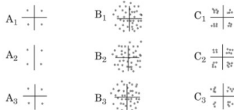
(b) Signal constellations.
