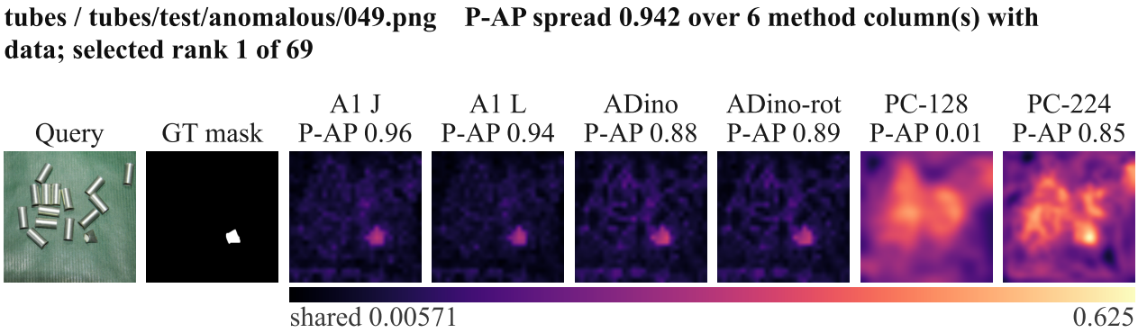
Figure 7 - mpdd tubes: multi-method per-sample comparison on the S8 common region (seed 0, K 4; region 392 x 392, 76.6% of the canvas)
