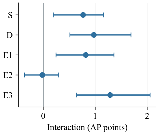
(a) MPDD I_{\text{TRI}}
