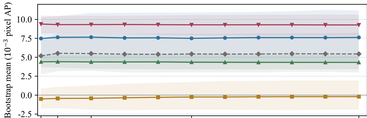
(a) Prefix estimate and 95% percentile interval: I_{\text{TRI}}
