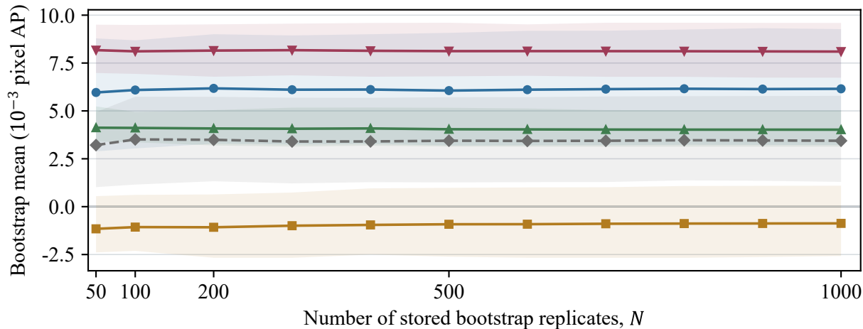
(b) Prefix estimate and 95% percentile interval: I_{\text{BAL}}
