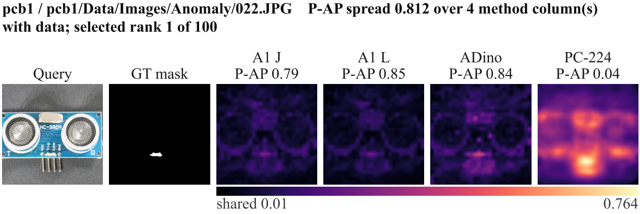
Figure 7 - visa pcb1: multi-method per-sample comparison on the S8 common region (seed 0, K 4; region 392 x 393, 59.8% of the canvas)
